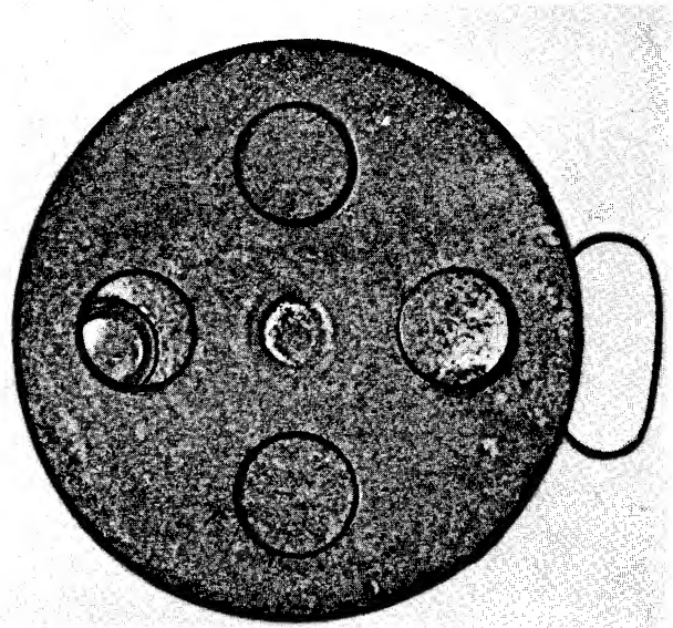
Figure 7. Chinese Communist antitank mine.
